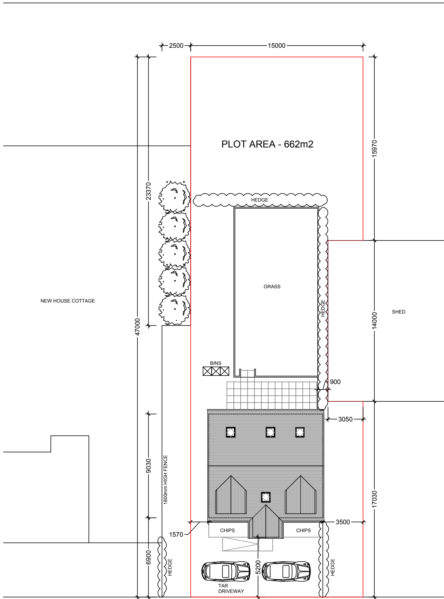
BLOCK PLAN AS PROPOSED 1:200
