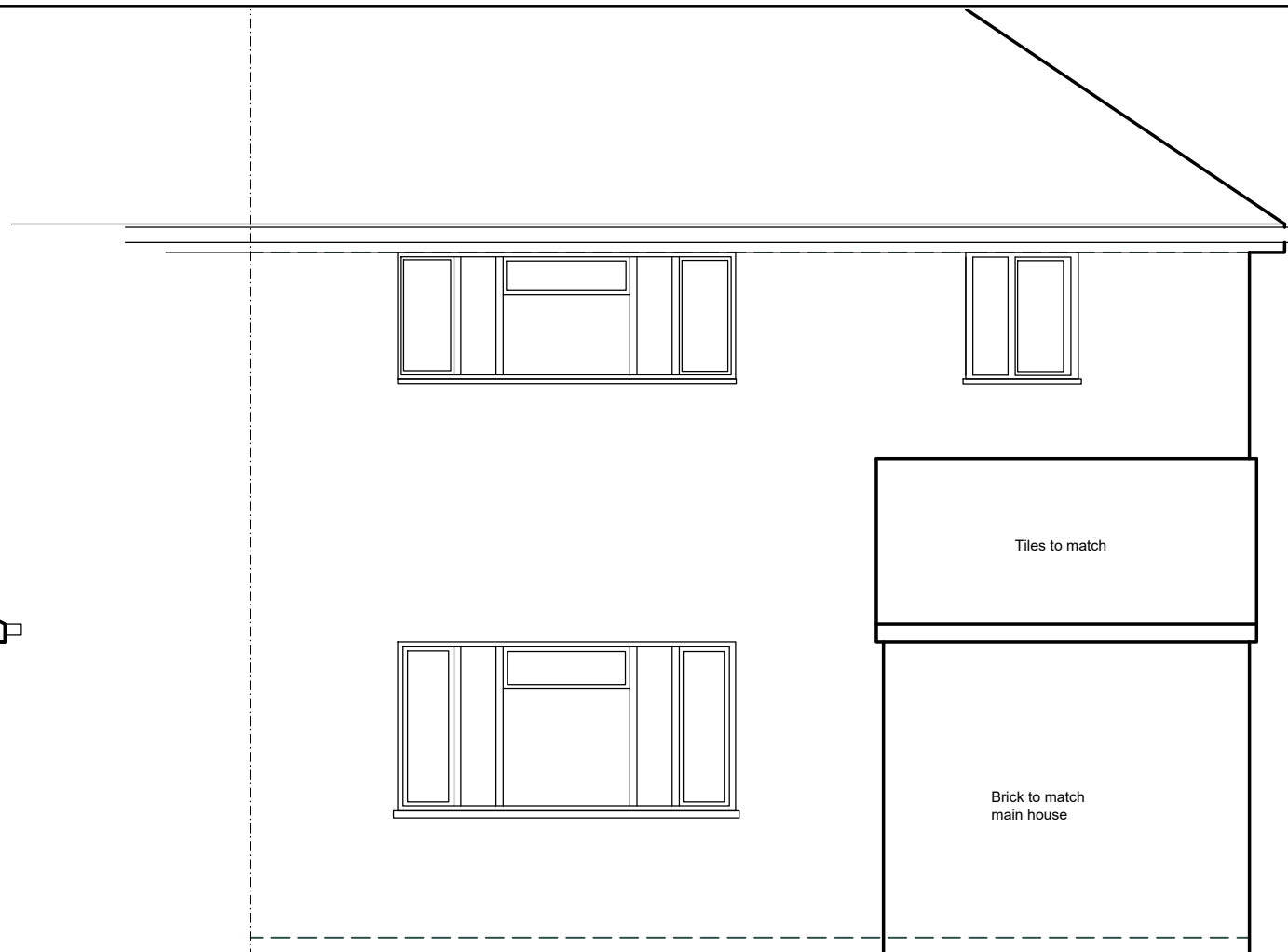
Proposed Front Elevation 1:50 Scale
