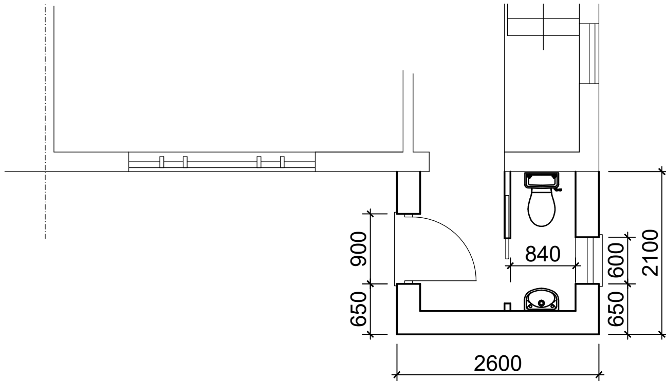
Proposed Ground floor 1:50 Scale
