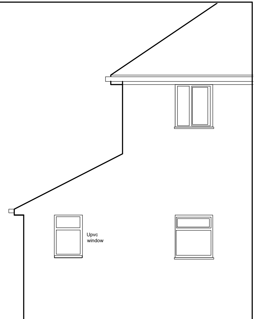
Proposed boundary Elevation (Part) 1:50 Scale
