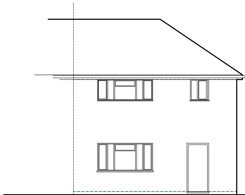
Existing Front Elevation 1:100 Scale
