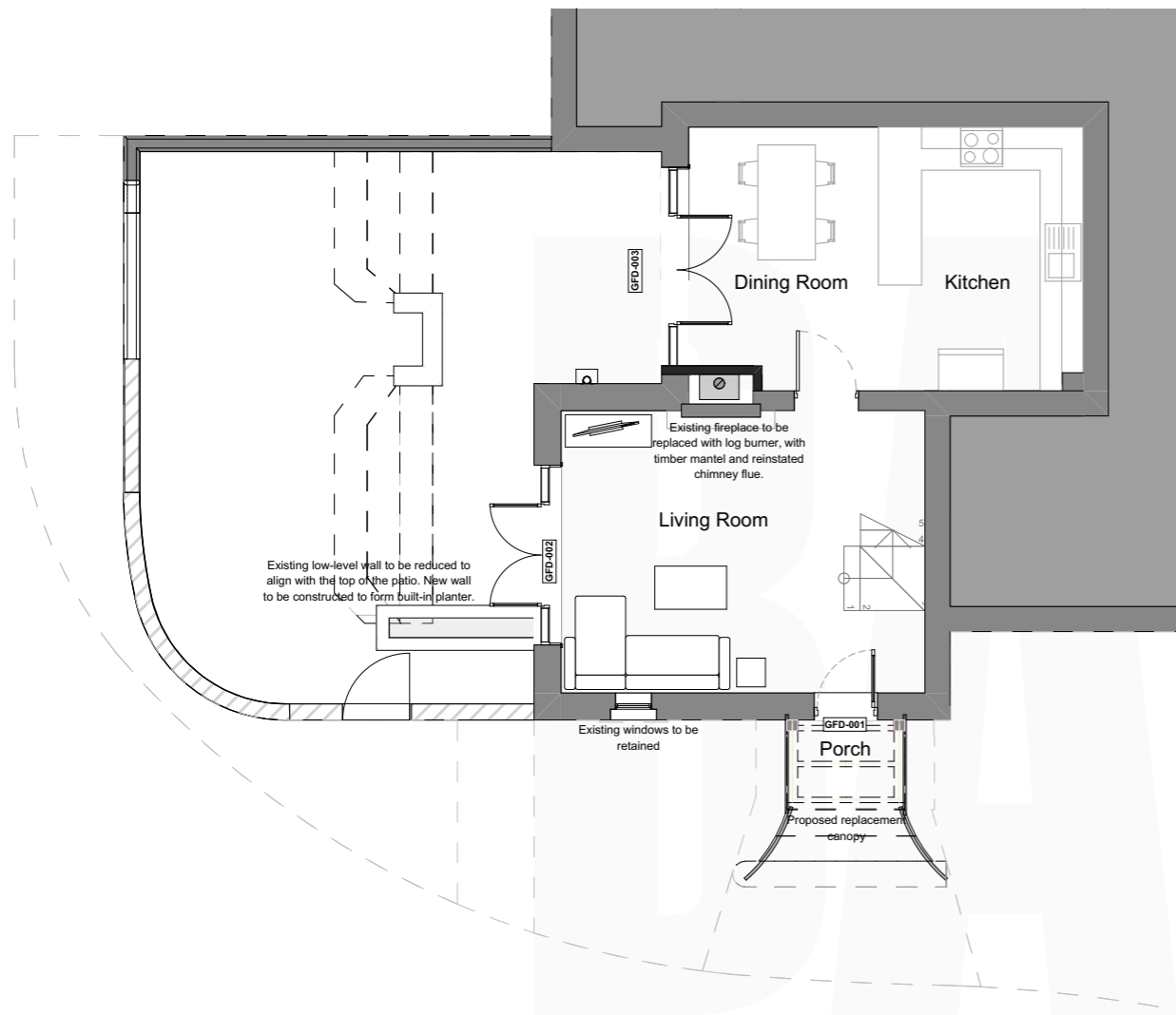
Ground Floor 1:100
