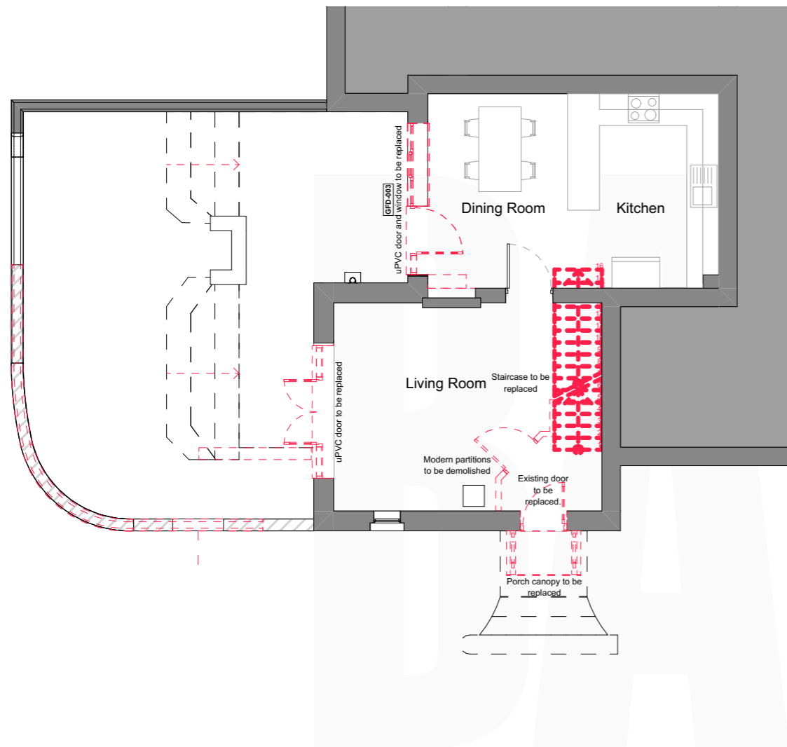
Ground Floor - Demolition Plan 1:100
