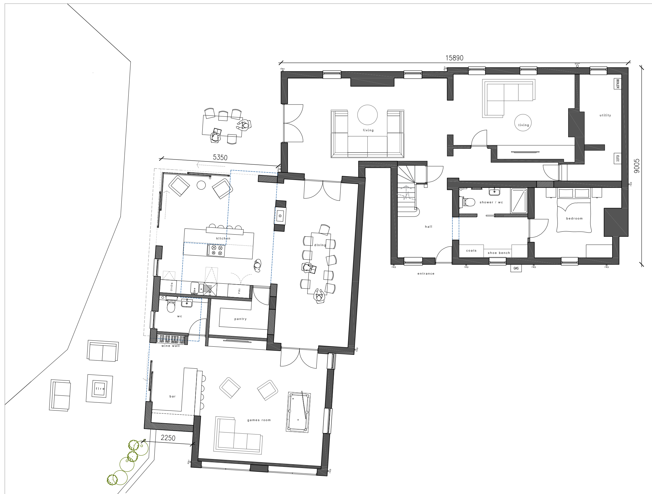
- Ground Floor
