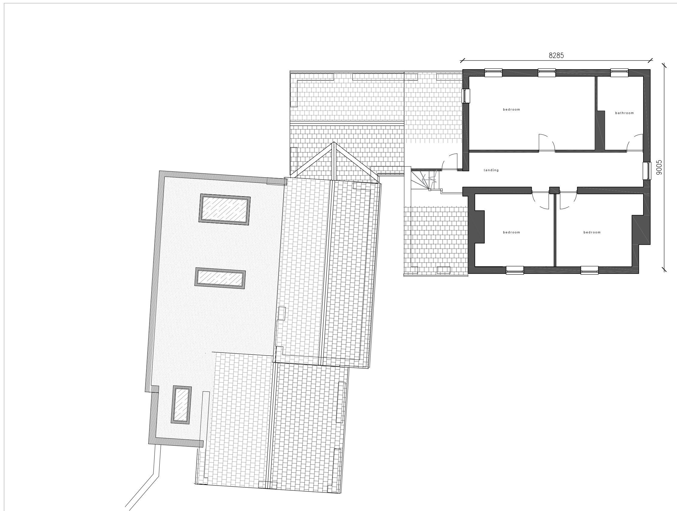
- First Floor + Roof Layout
