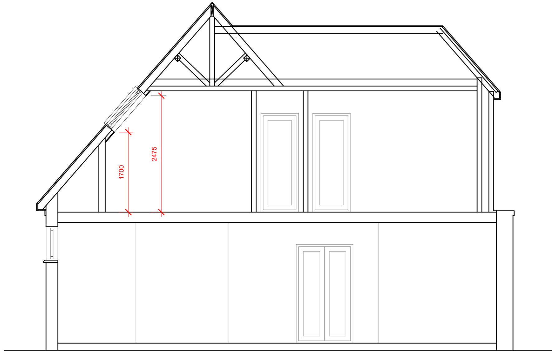
Proposed Section Scale 1:50
