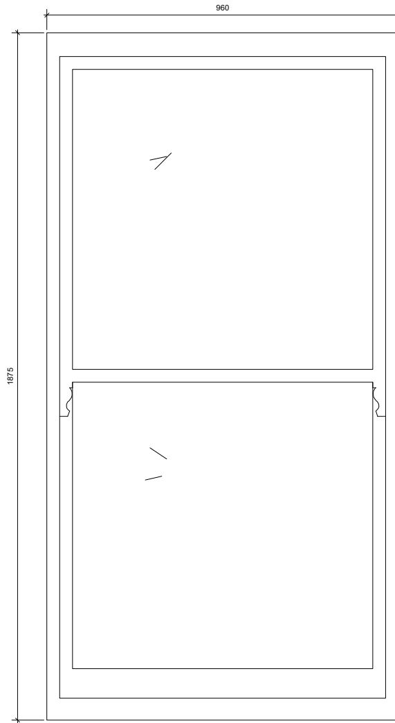
Window F Elevation 1:5 @A1, 1:10@A3
