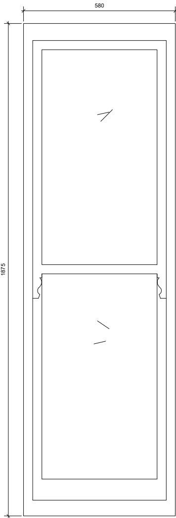
Window E and G Elevation 1:5 @A1, 1:10@A3
