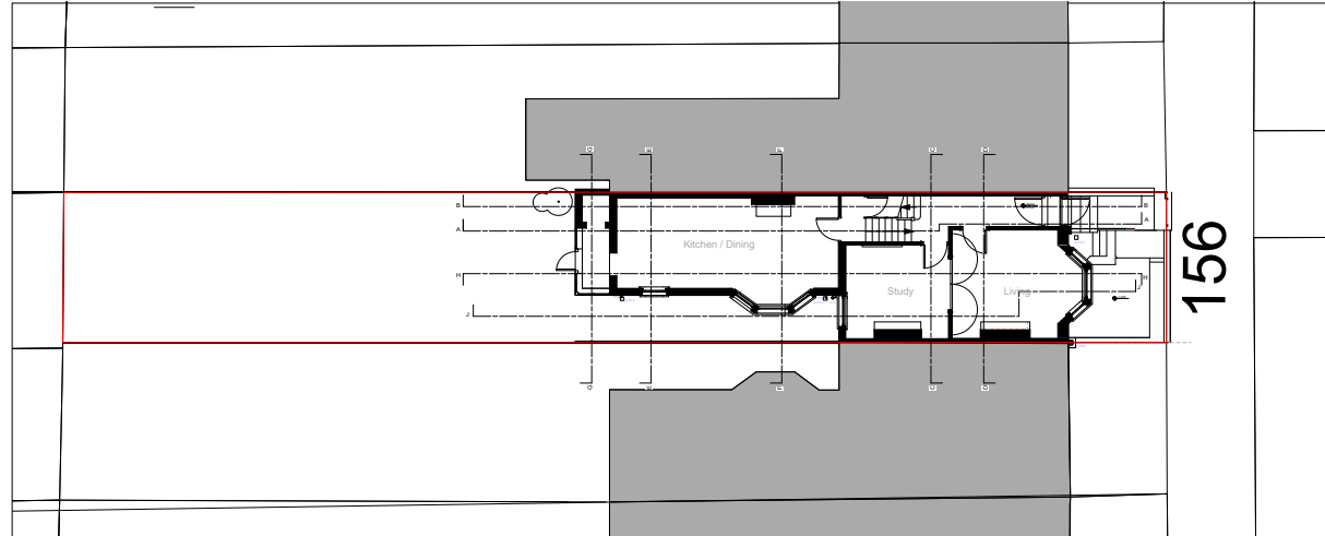
Existing Ground Floor Block Plan 1:100@A1, 1:200@A3
