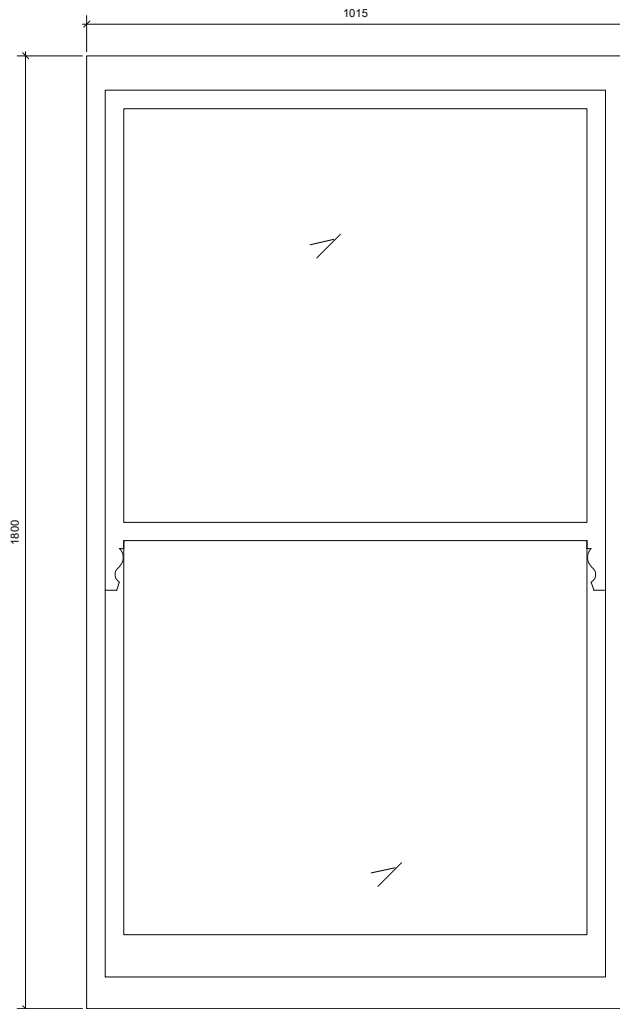
Window L Elevation 1:5 @A1, 1:10@A3
