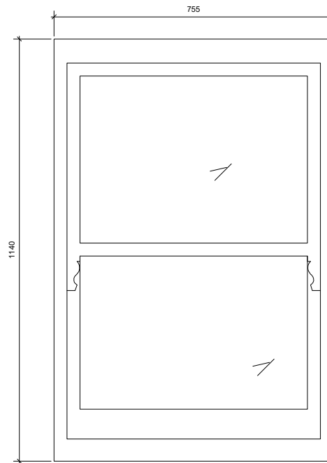
Window M Elevation 1:5 @A1, 1:10@A3
