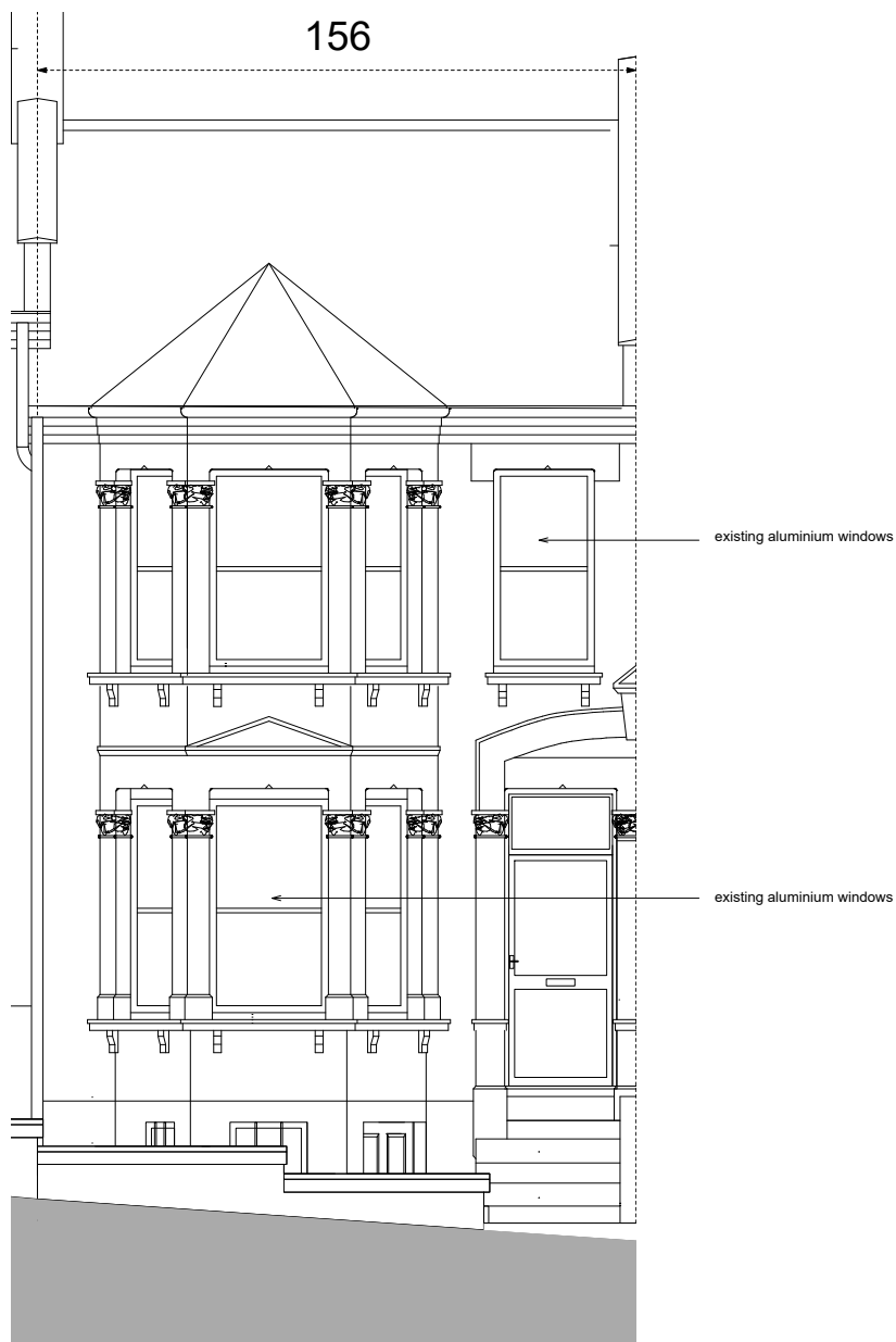
Front (East) Elevation Existing 1:25@A1, 1:50 @ A3
