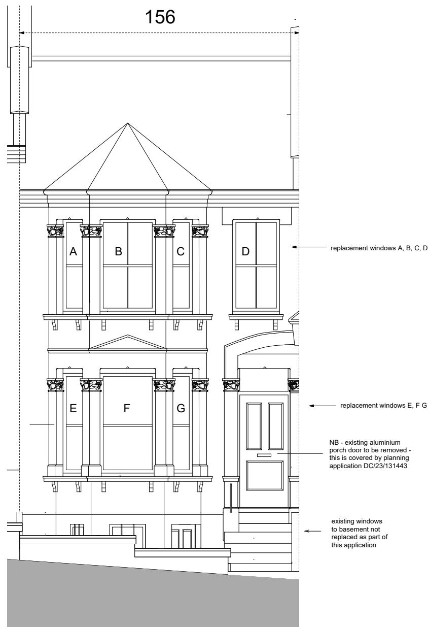
Front (East) Elevation Proposed 1:25@A1, 1:50 @ A3
