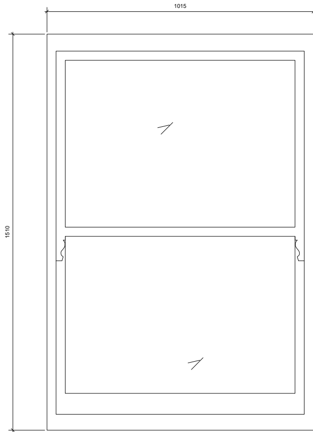
Window K Elevation 1:5 @A1, 1:10@A3
