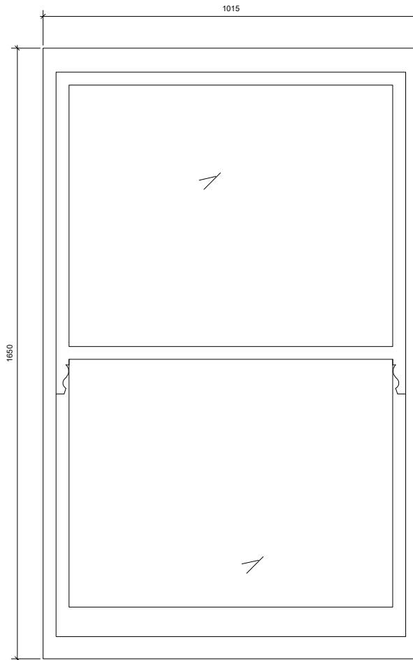
Window J Elevation 1:5 @A1, 1:10@A3
