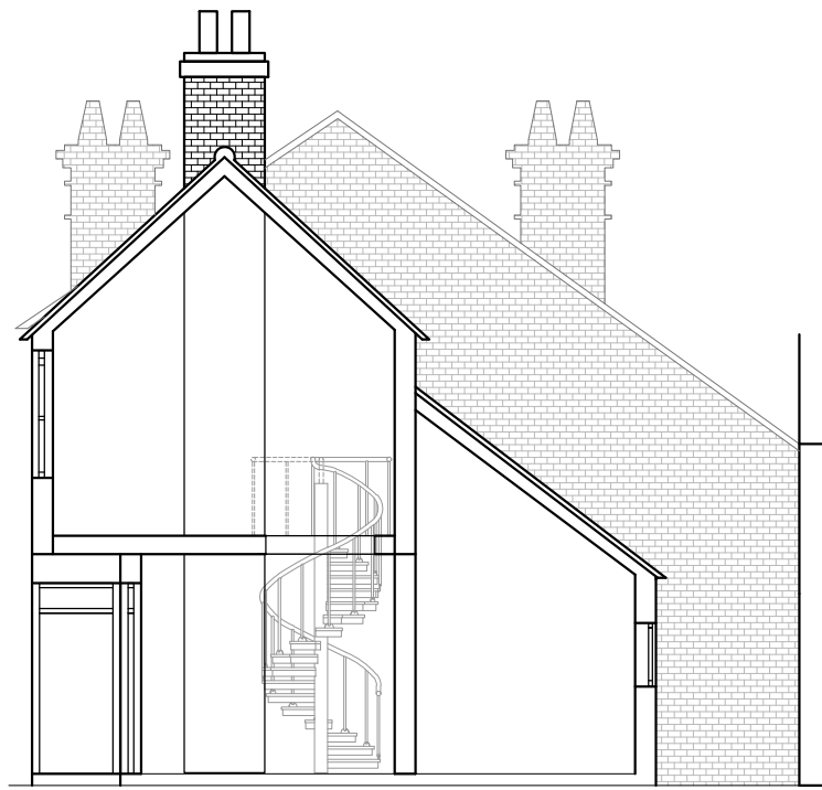
EXISTING A-A SECTION
