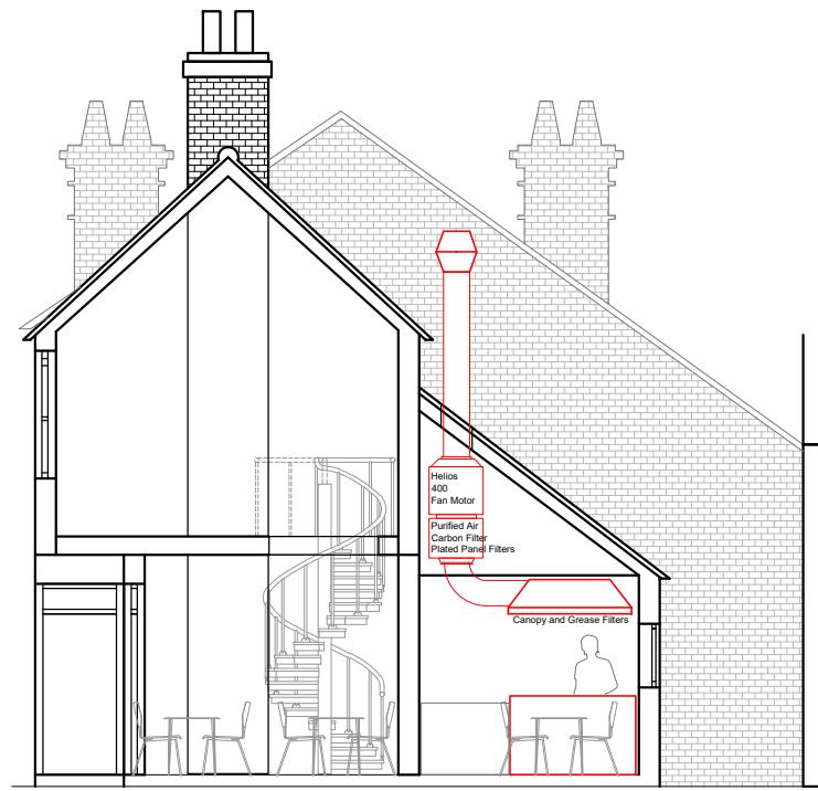
PROPOSED A-A SECTION
