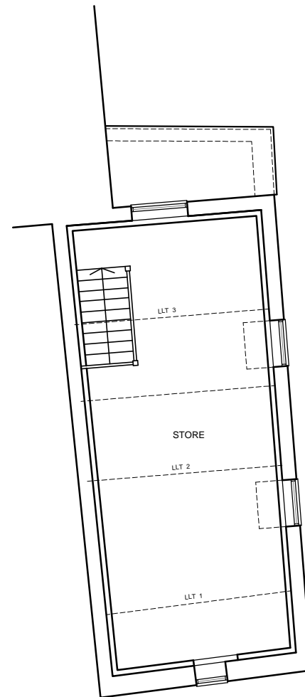
FIRST FLOOR PLAN (OVER KITCHEN)
