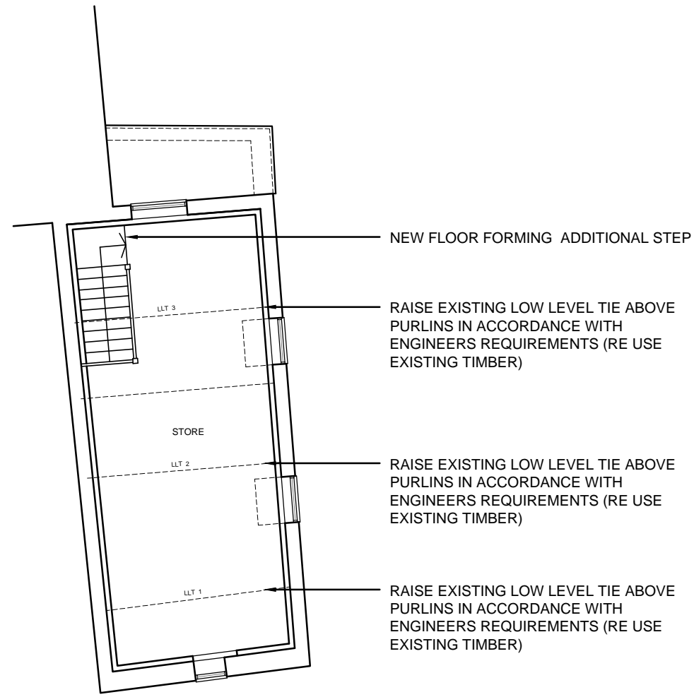
FIRST FLOOR PLAN (OVER KITCHEN)
