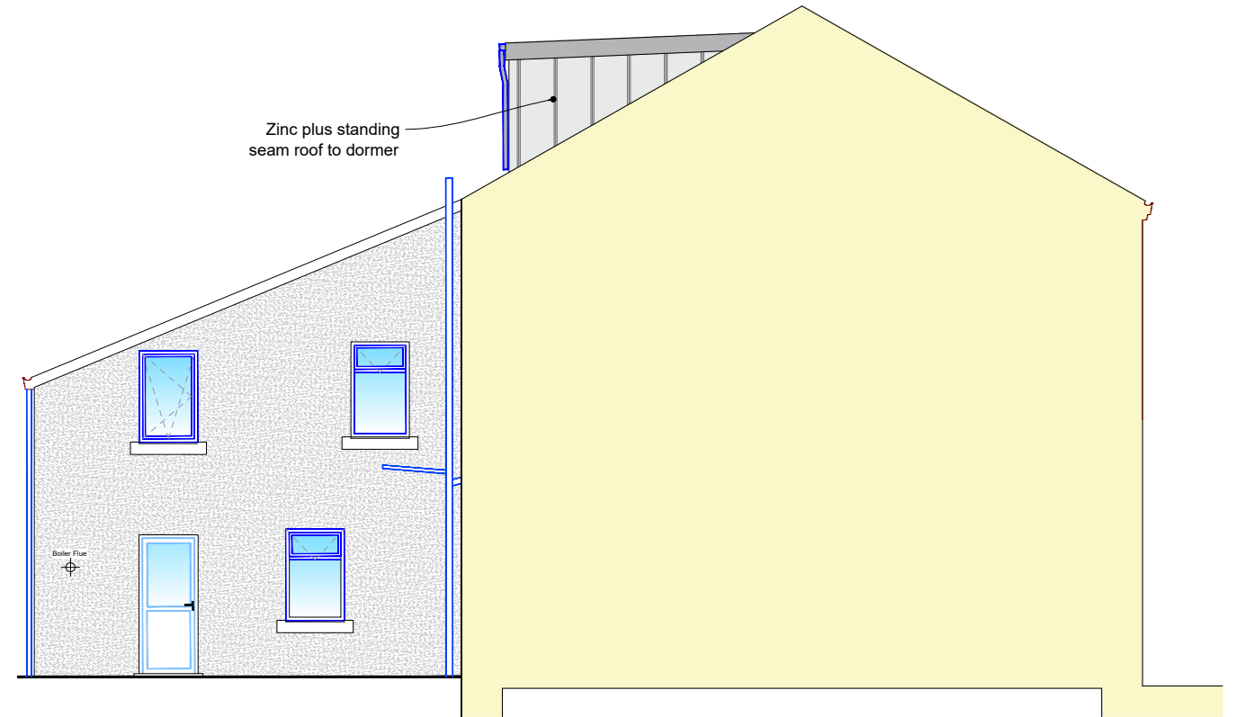
Side Elevation as Proposed Scale: 1/100 @ A3
