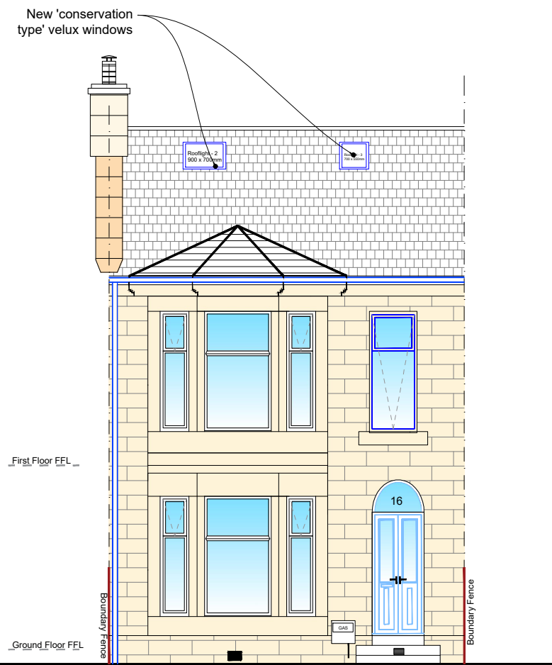
Front Elevation as Proposed Scale: 1/100 @ A3
