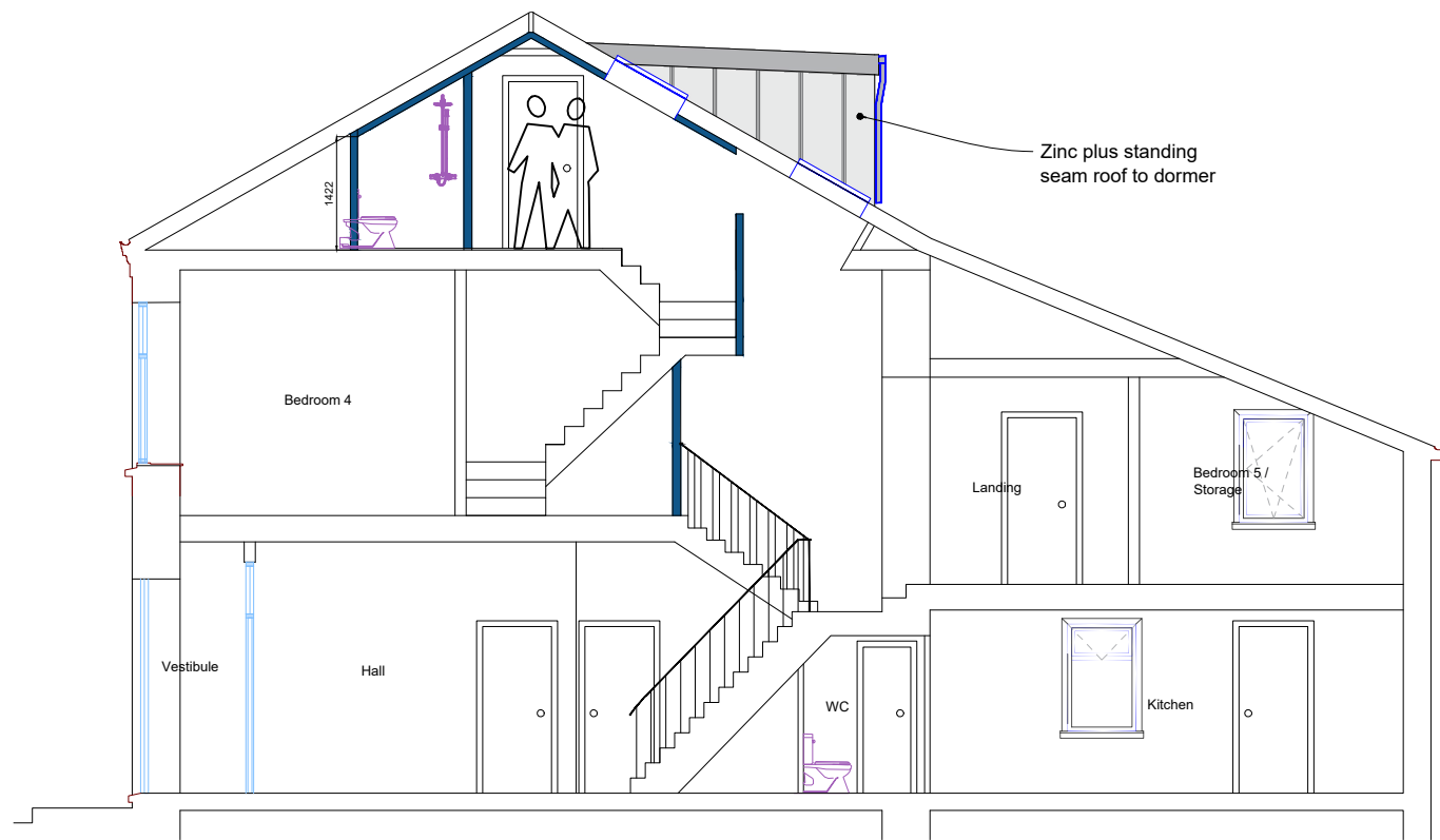
Section through A-A as Proposed North Facing Dormer Elevation Scale: 1/100 @ A3
