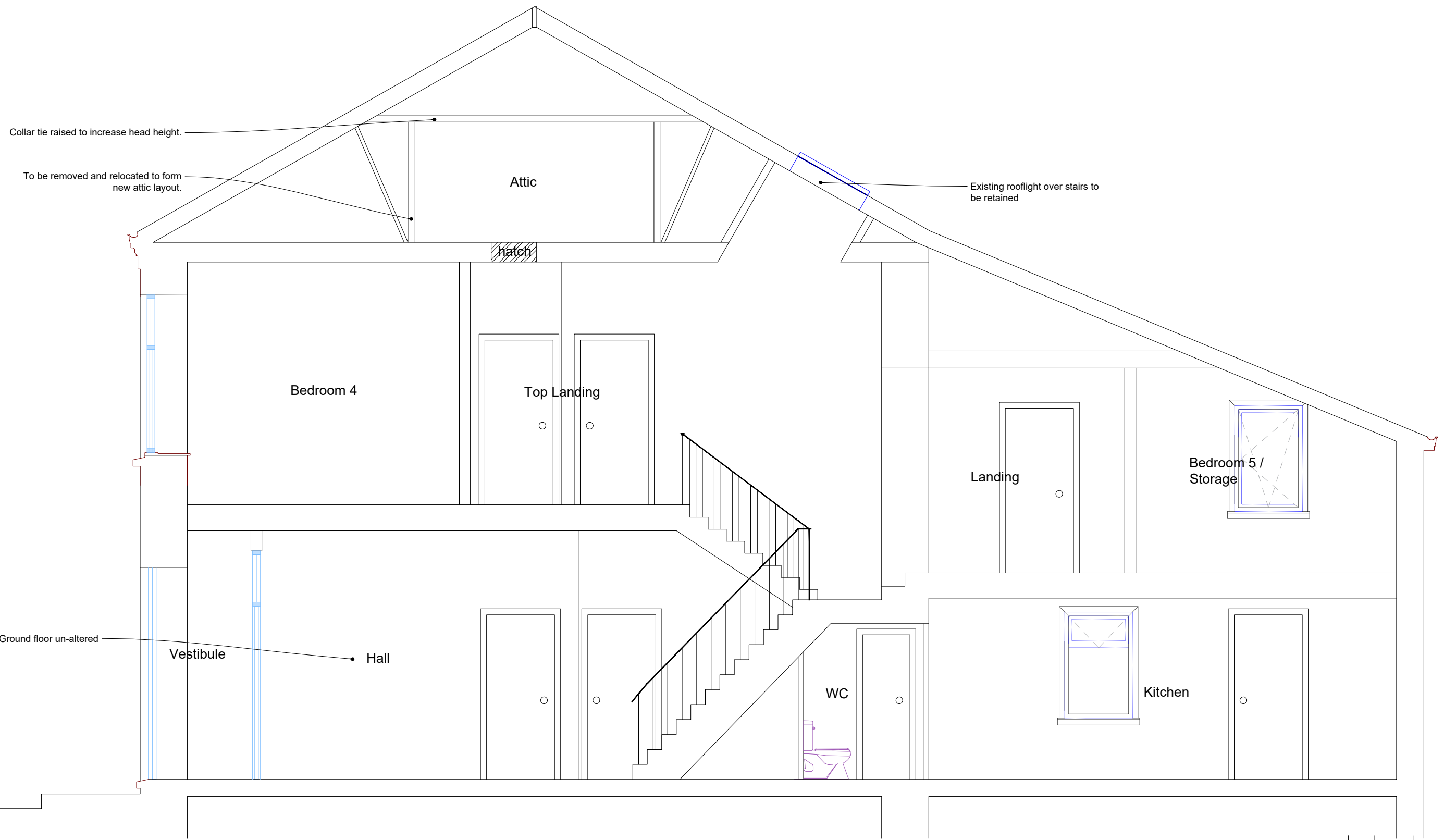
Section Through A-A as Existing Scale: 1/50 @ A3
