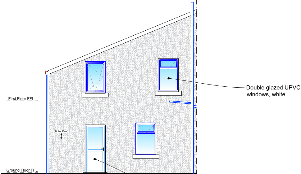
Side Elevation as Existing Scale: 1/100 @ A3
