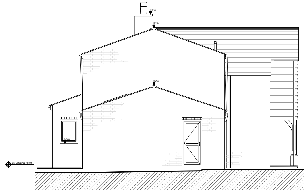
4 SIDE (NE) ELEVATION
