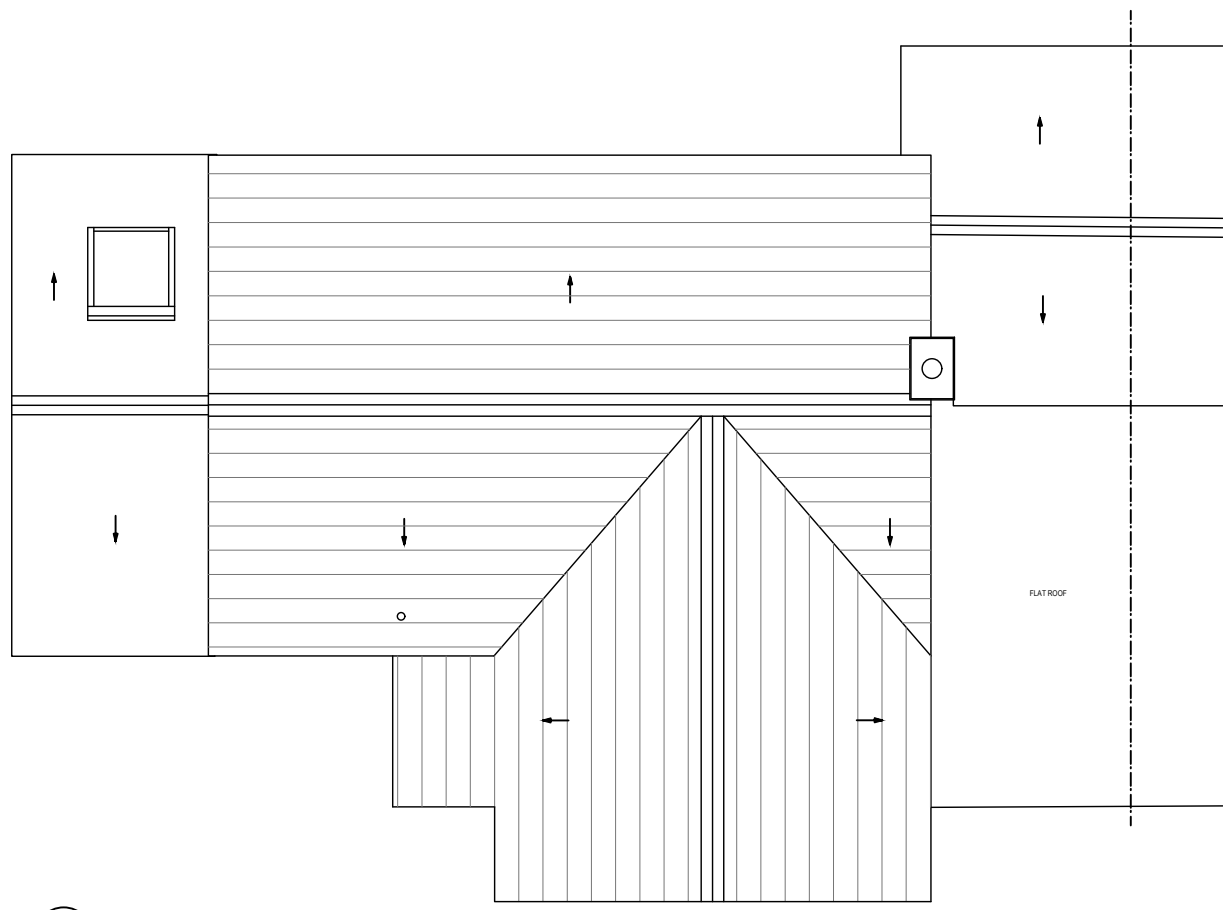
3 ROOF PLAN 03
