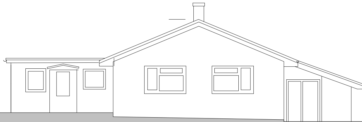
2 Existing Elevation Facing North 1 : 100
