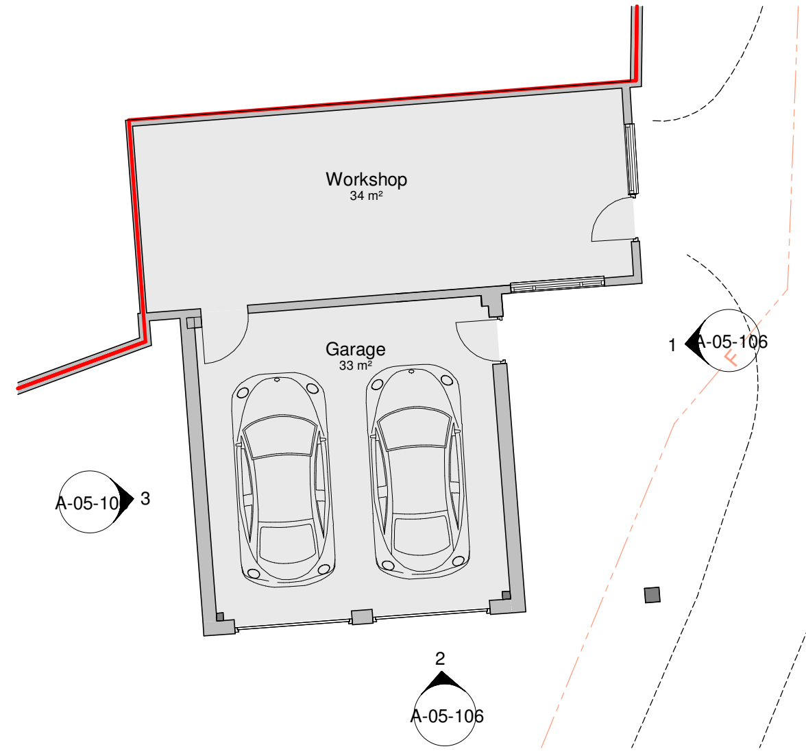
4 0.00 Proposed Garage Plan 1 : 100
