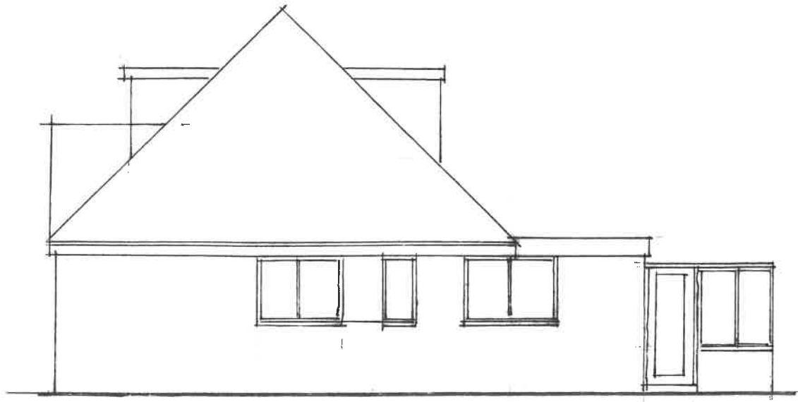
EXISTING SIDE ELEVATION. [SOUTH WEST.]
