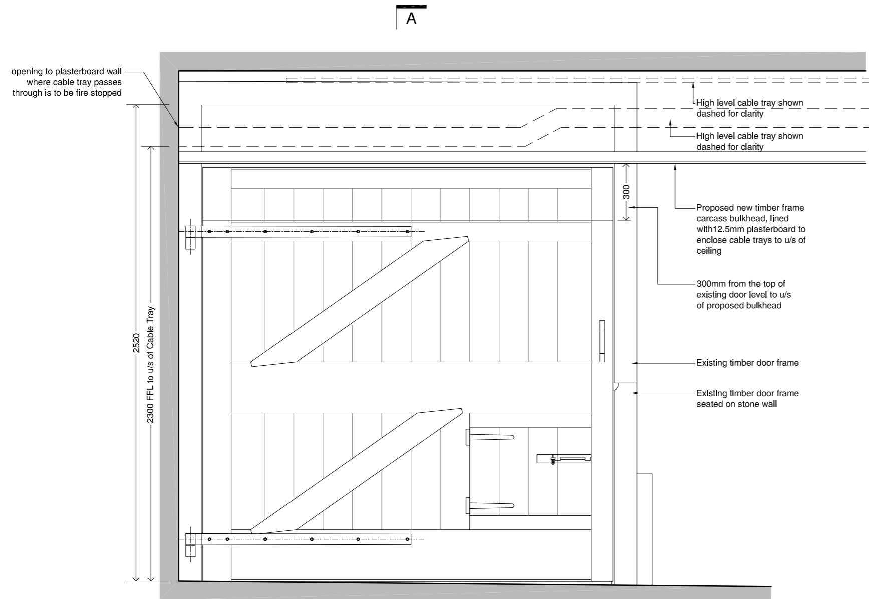
04 Proposed Inner Door to Still Room Scale 1:20 Elevation View
