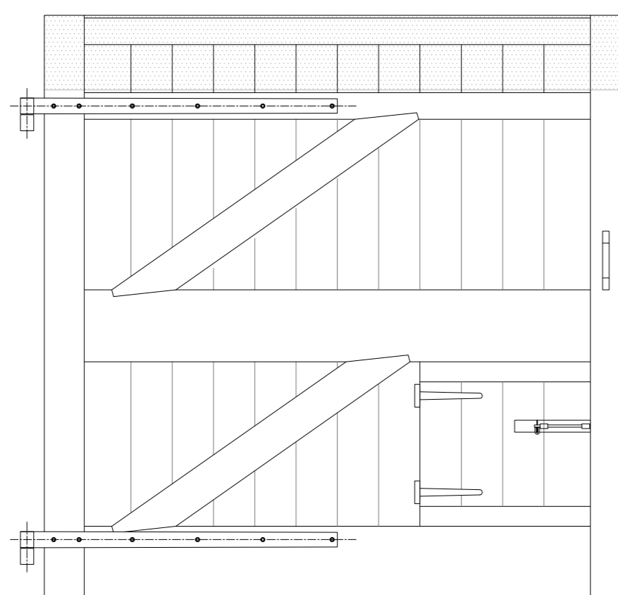
01 Proposed Inner Door to Still Room Scale 1:20 Corridor Side
