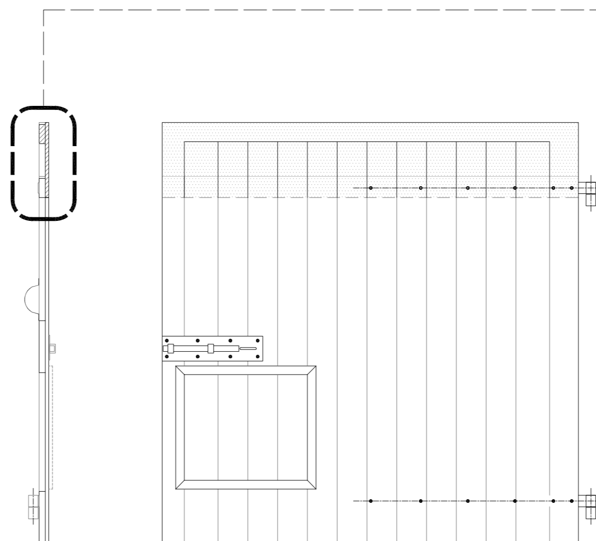
02 Proposed Inner Door to Still Room Scale 1:20 Still Room Side
