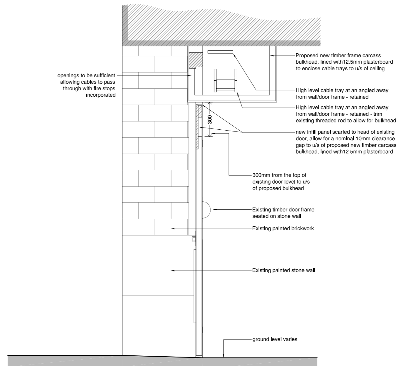
05 Proposed Inner Door to Still Room Scale 1:20 Section AA
