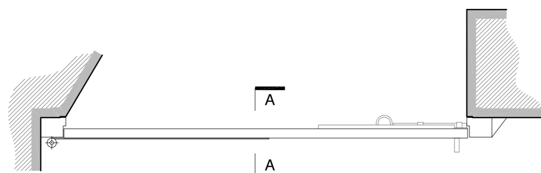
03 Proposed Inner Door to Still Room Scale 1:20 Plan View
