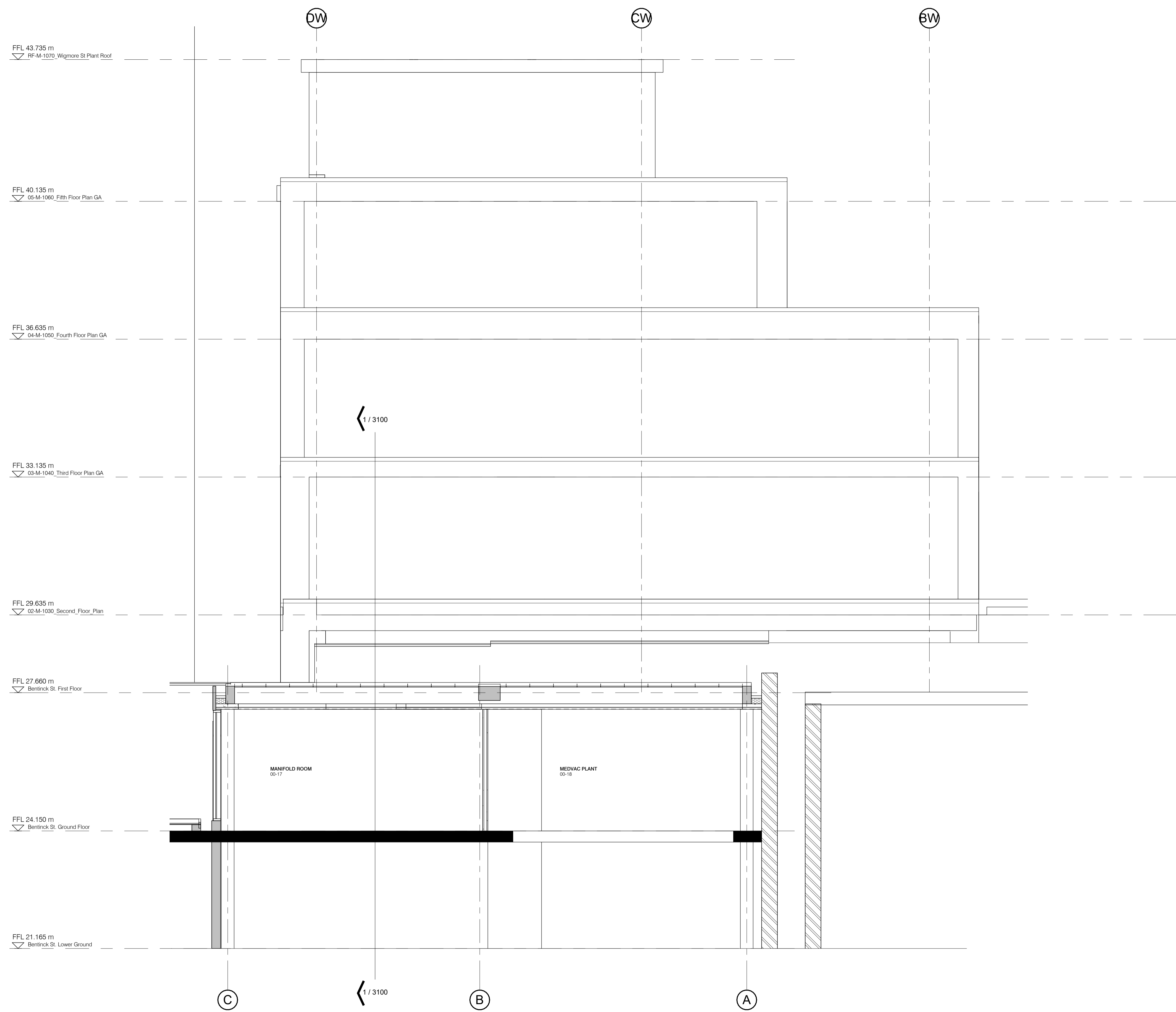
Existing Elevation 1 1 : 50
