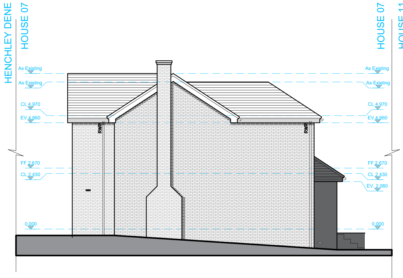
EXISTING NORTH WEST ELEVATION SCALE_1:100 AT A3
