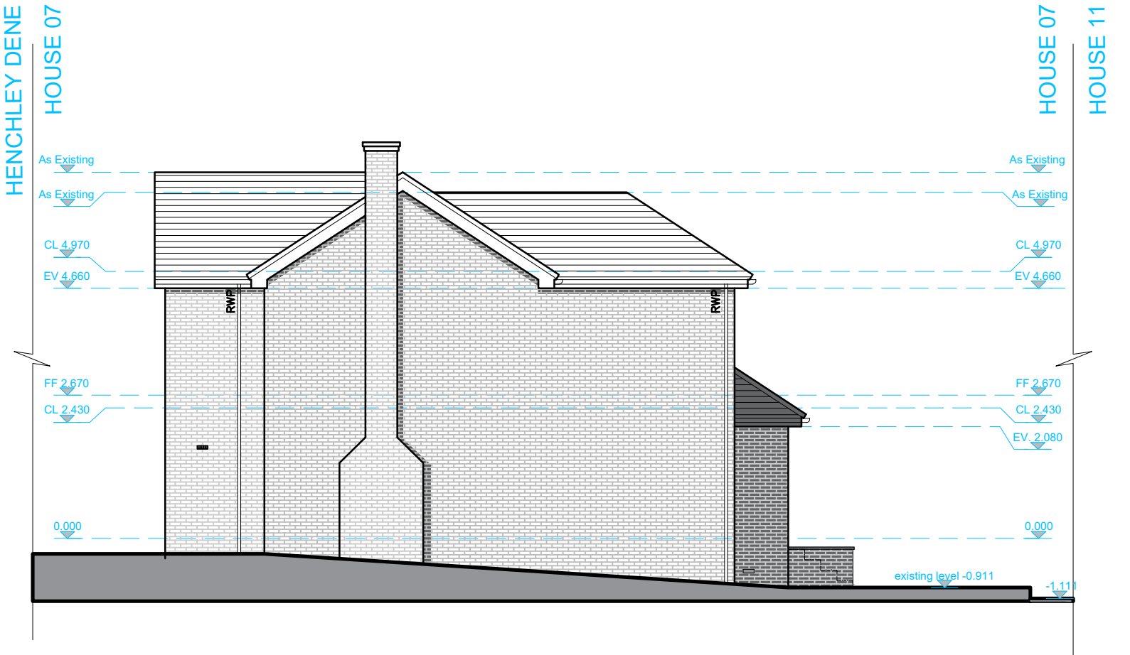
PROPOSED NORTH WEST ELEVATION SCALE_1:100 AT A3
