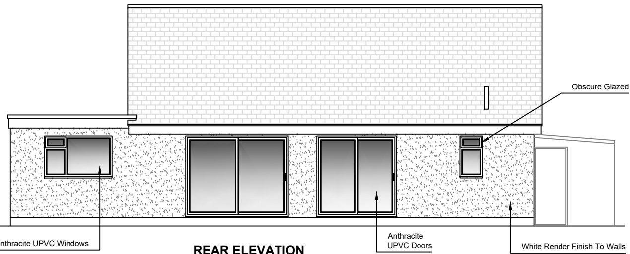
REAR ELEVATION
