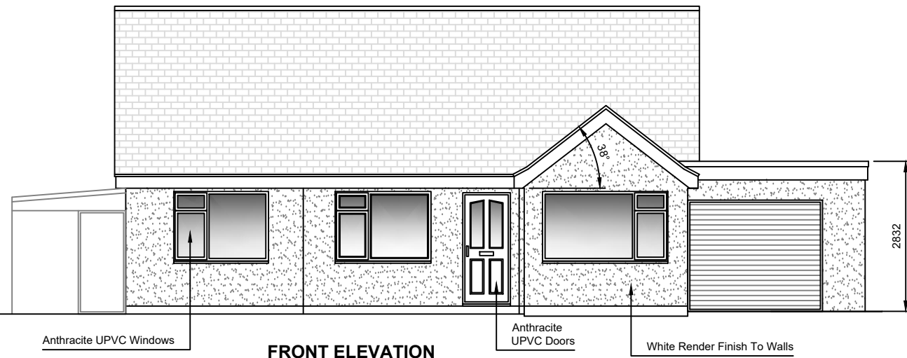
FRONT ELEVATION
