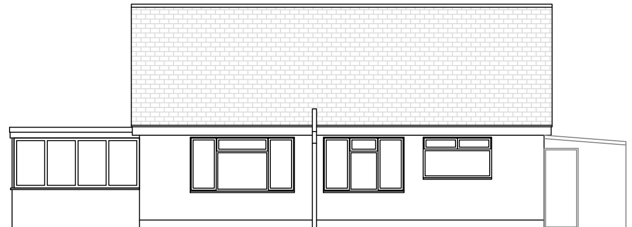
REAR ELEVATION
