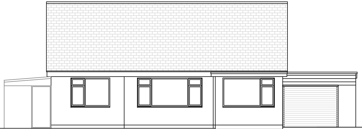
FRONT ELEVATION
