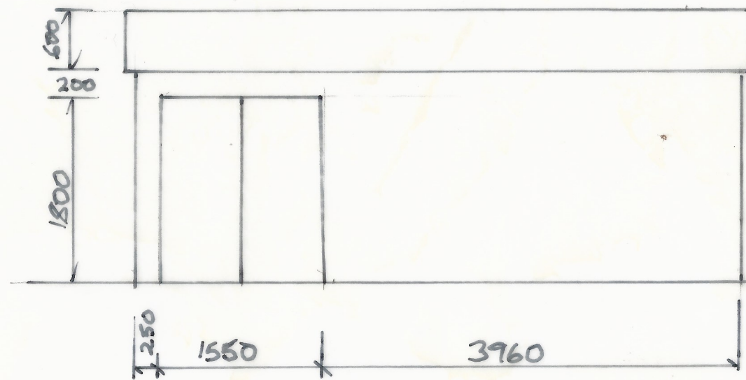
EAST ELEVATION (CAR PARK VIEW)
