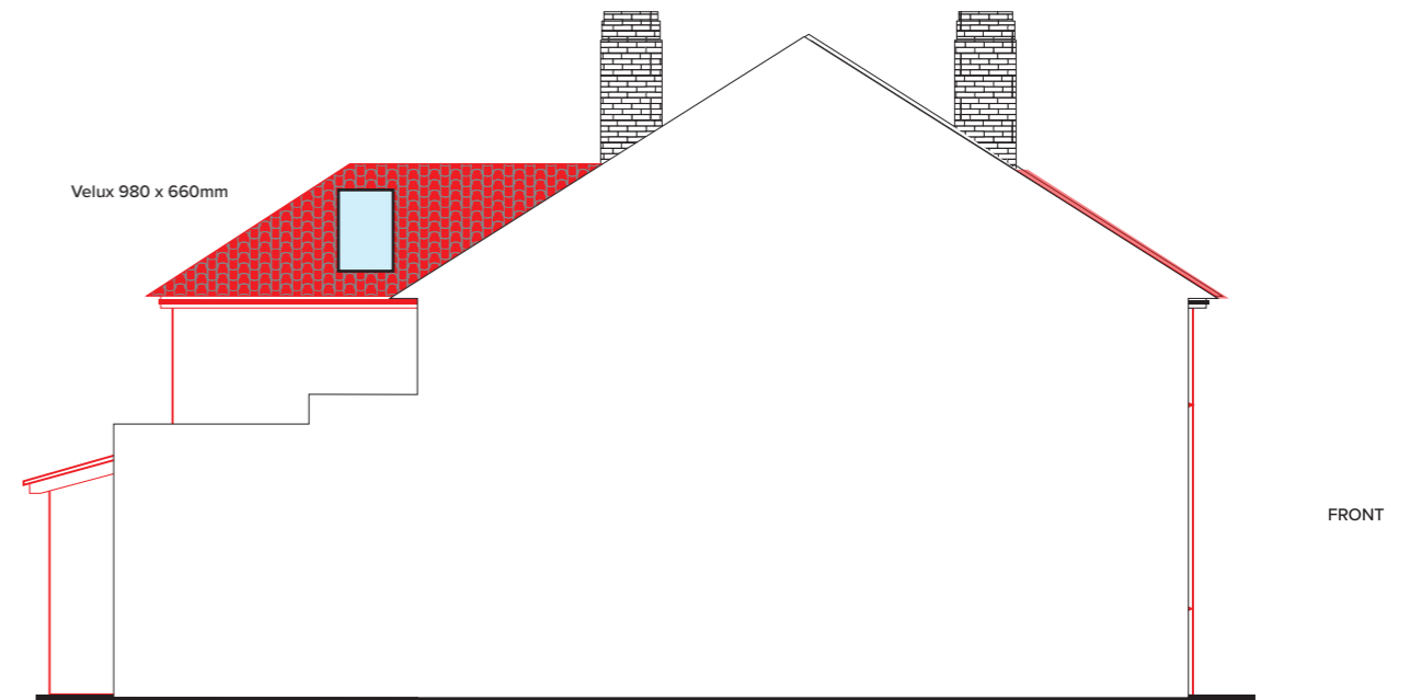
Proposed Party Wall Side Elevation
