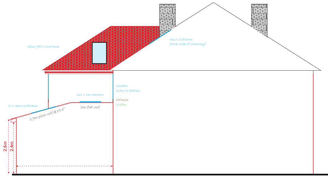
Proposed Ground Floor pitched roof and flat roof from Party Wall side view (I have removed the concrete garden wall for demonstration viewing purpose only)
