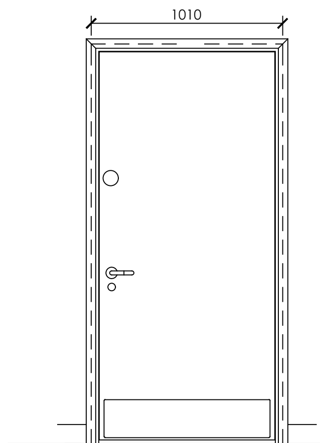
Type A - Internal Flush, Single door
