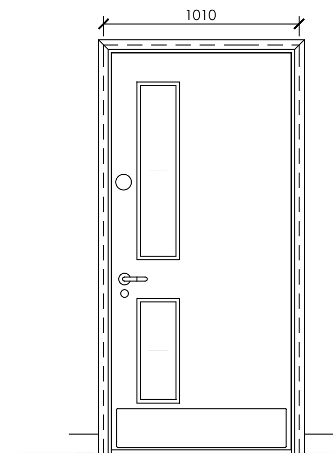
Type B - Internal Flush, Single Door
