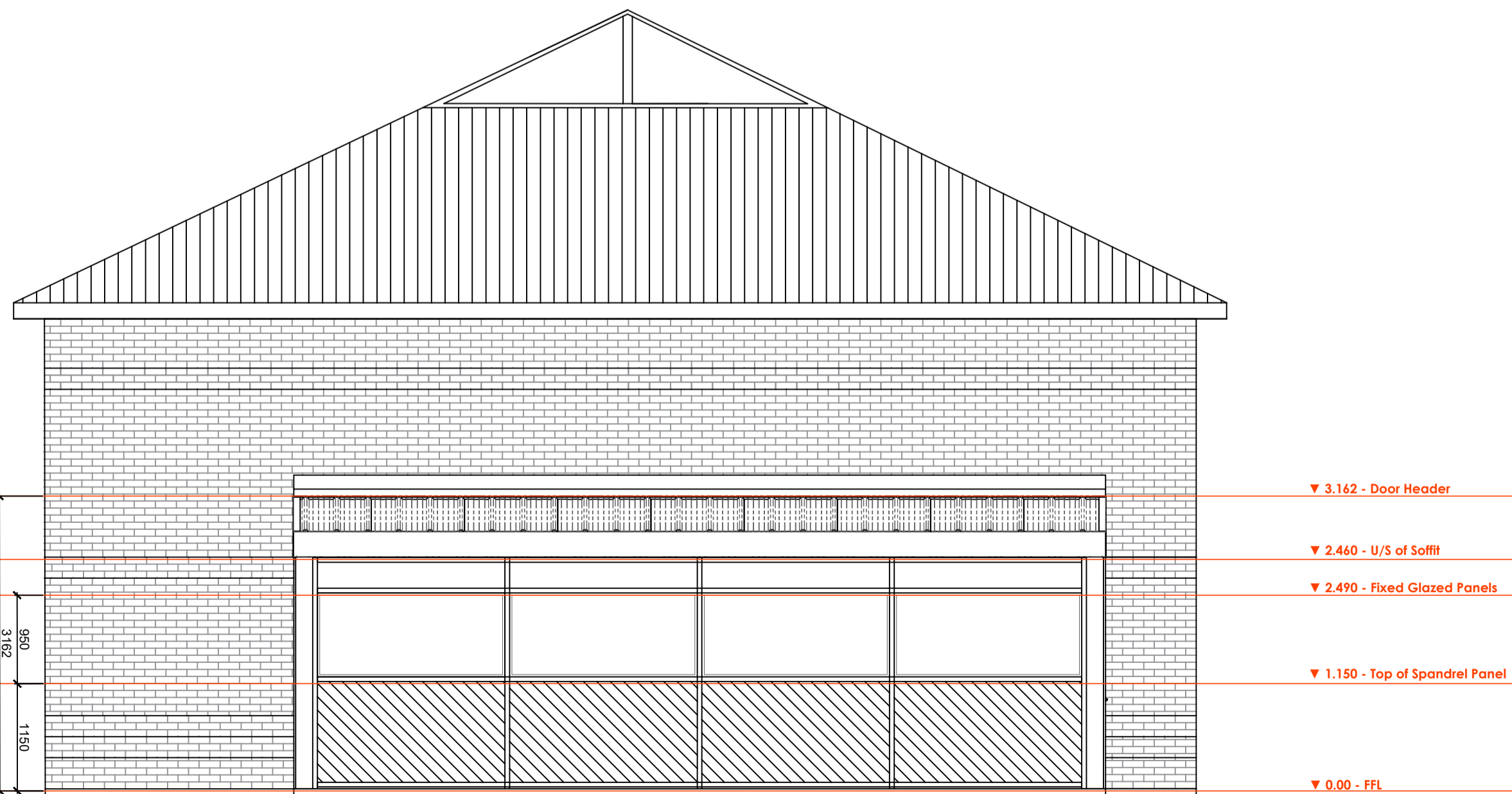
Proposed Elevation - North West
