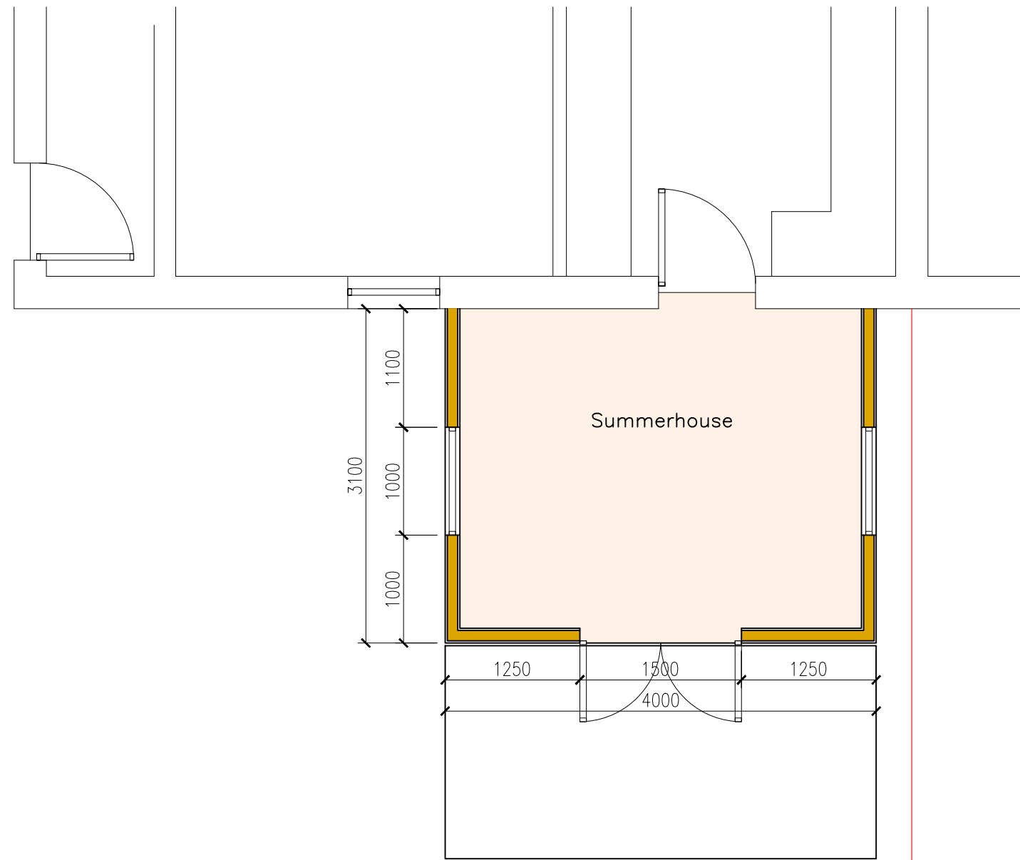
Proposed Floor Plan 1:50
