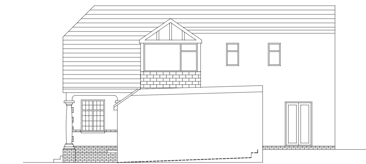
Side Elevation (South West)
