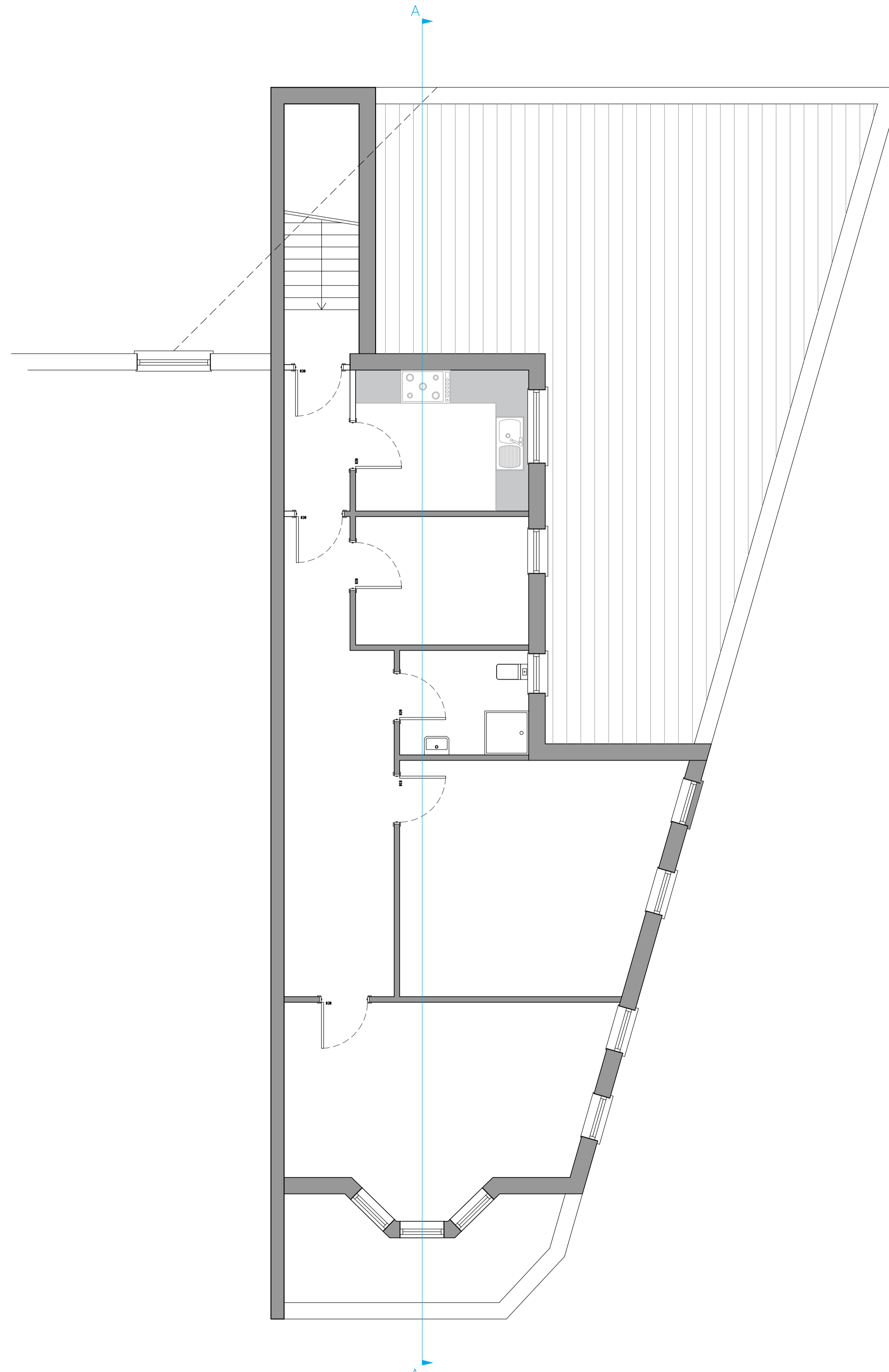
AS APPROVED FIRST FLOOR PLAN ALL NEIGHBORING PROPERTIES ARE INDICATIVE ONLY
