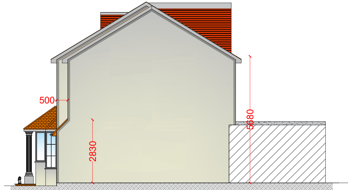
Proposed flank elevations 1:100
