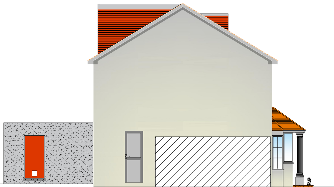
Existing West Facing Elevation 1:100
