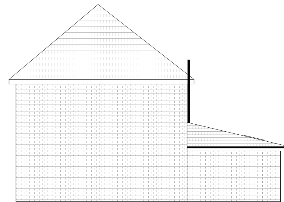
PROPOSED NEIGHBOURING SIDE ELEVATION
