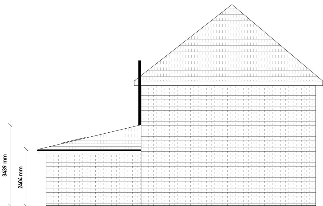
PROPOSED SIDE ELEVATION ATACHED
