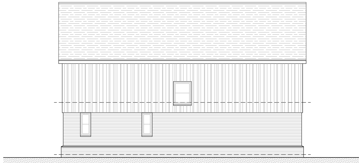
Side (North-East) Elevation 1:100
