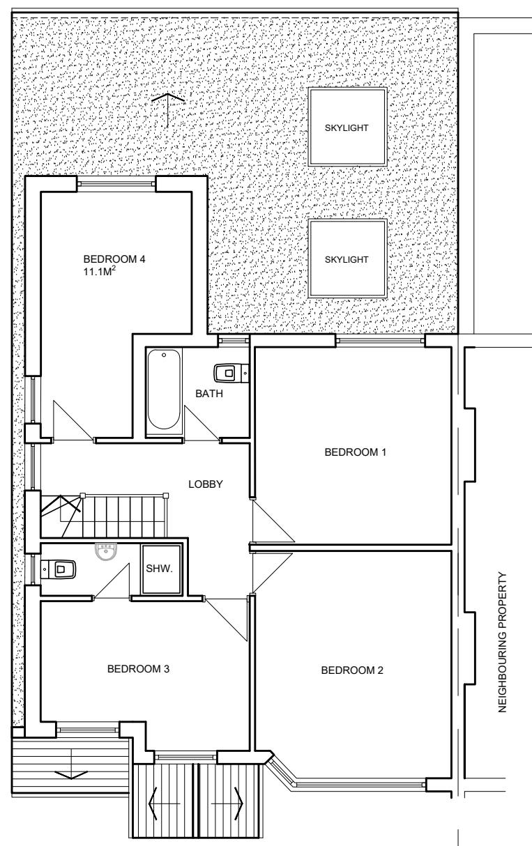
PREVIOUSLY APPROVED FIRST FLOOR PLAN
