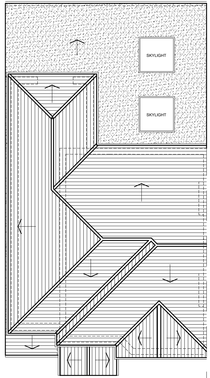
PREVIOUSLY APPROVED ROOF PLAN
