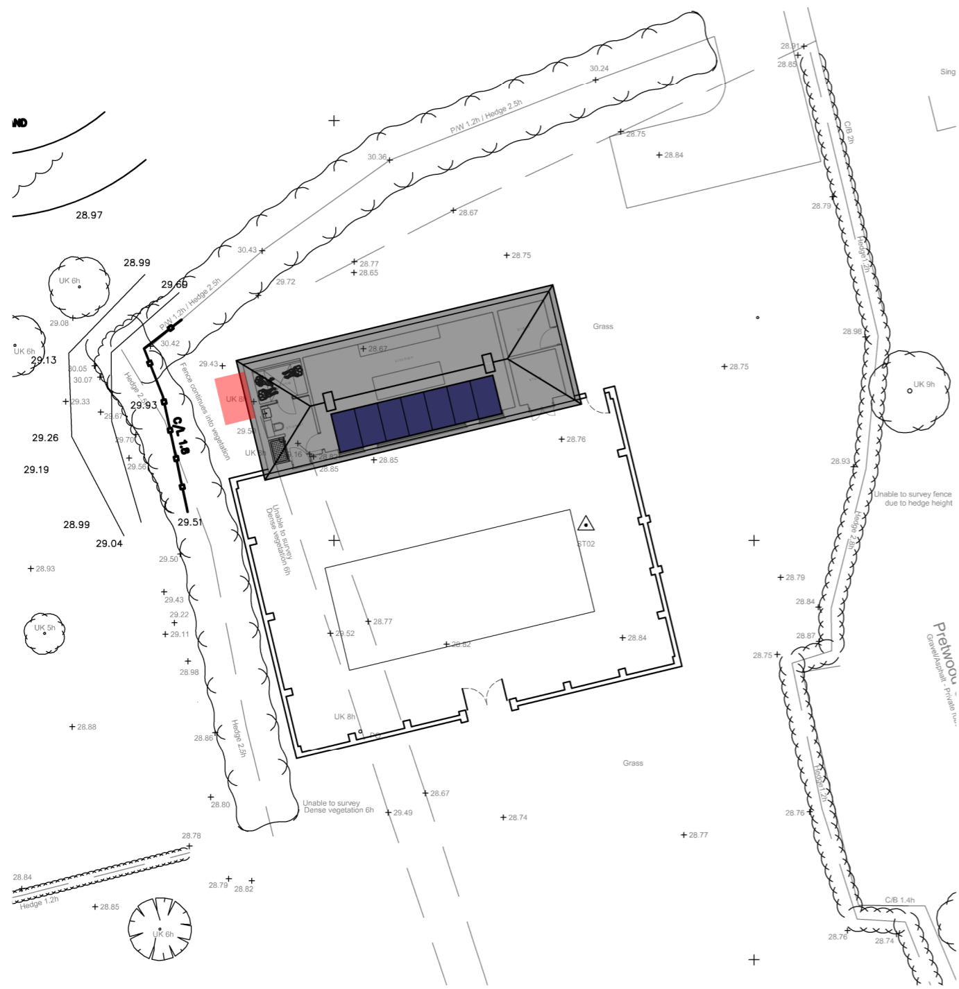
existing plan - 1:250
