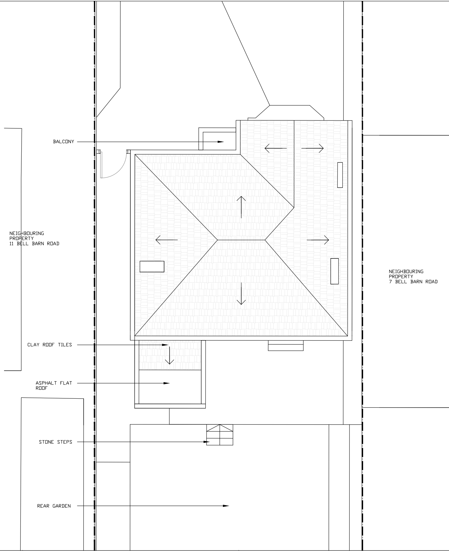
ROOF PLAN - EXISTING SCALE 1:100
