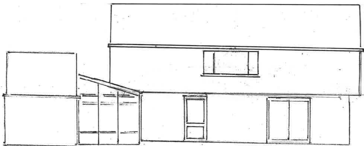
Proposed side Elevation North Facing
