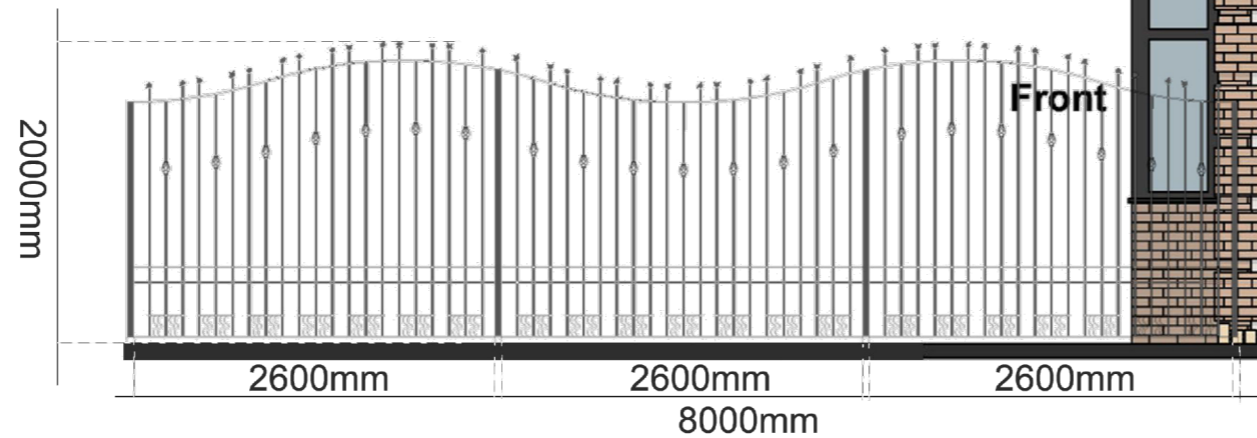
Proposed North West Facing Elevation Elevation
