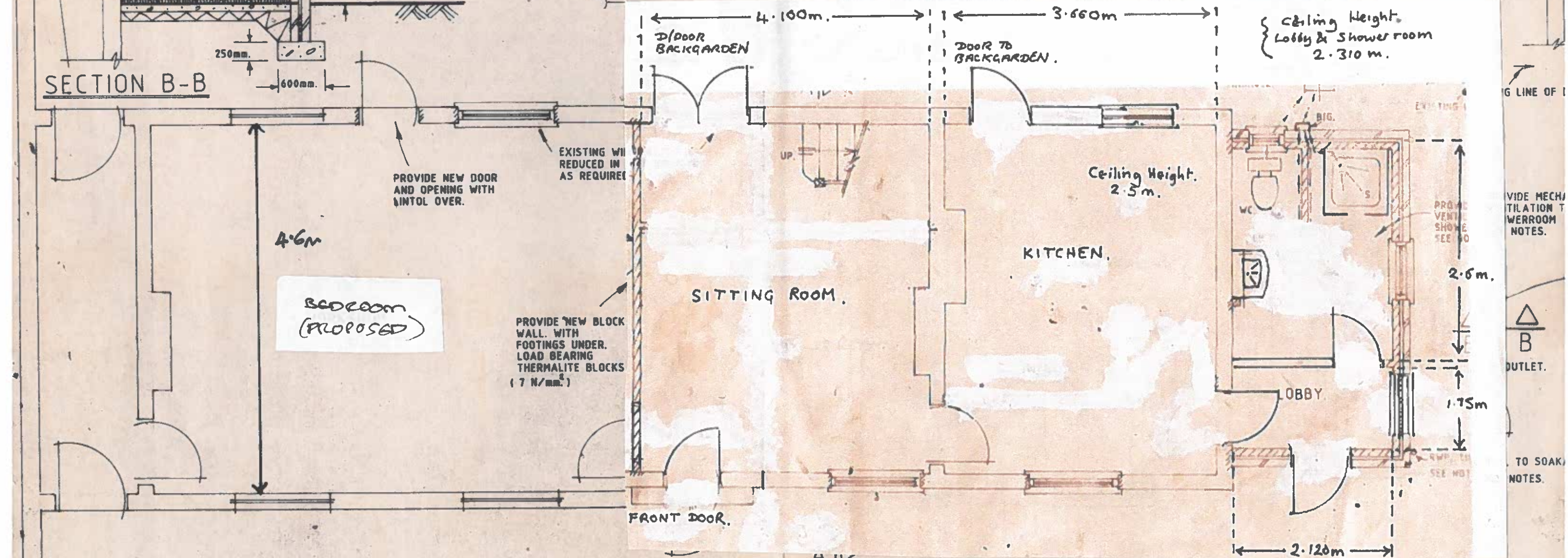
PROPOSED GROUND FLOOR
