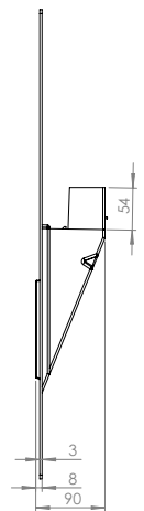
Side Profile
