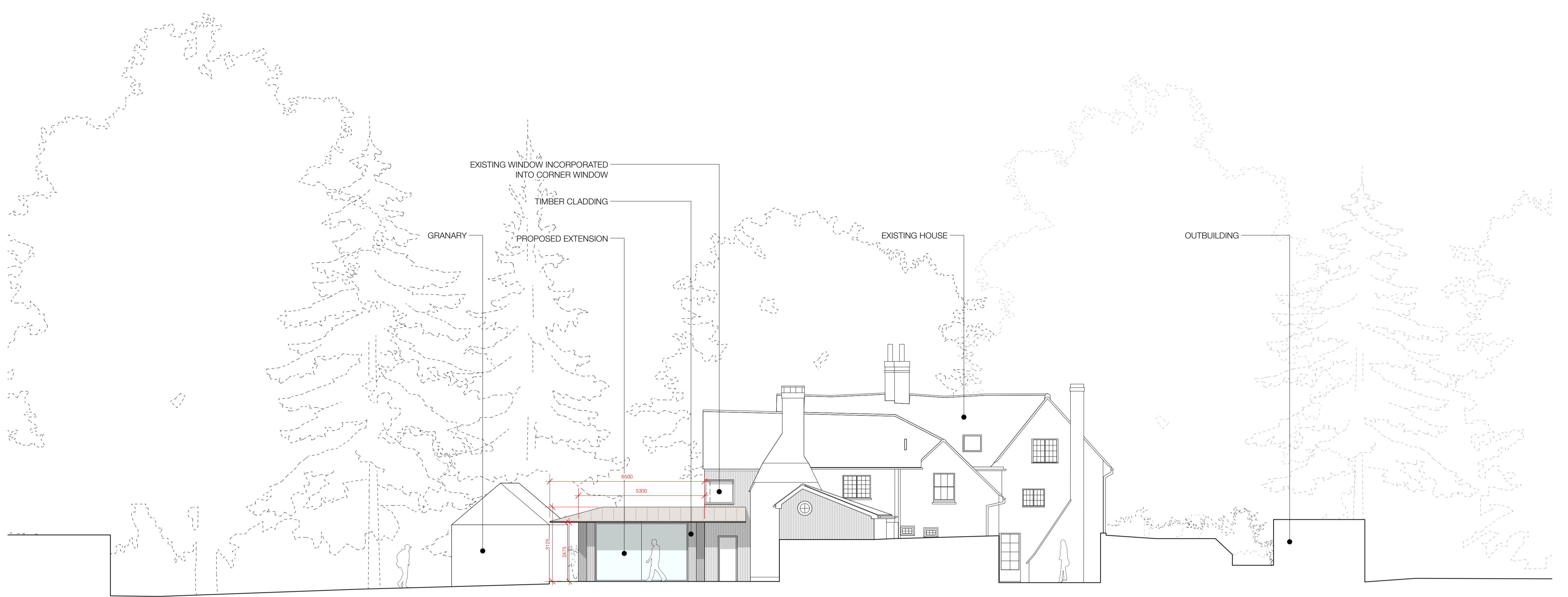
01 PROPOSED SOUTHERN ELEVATION Scale: 1:100
