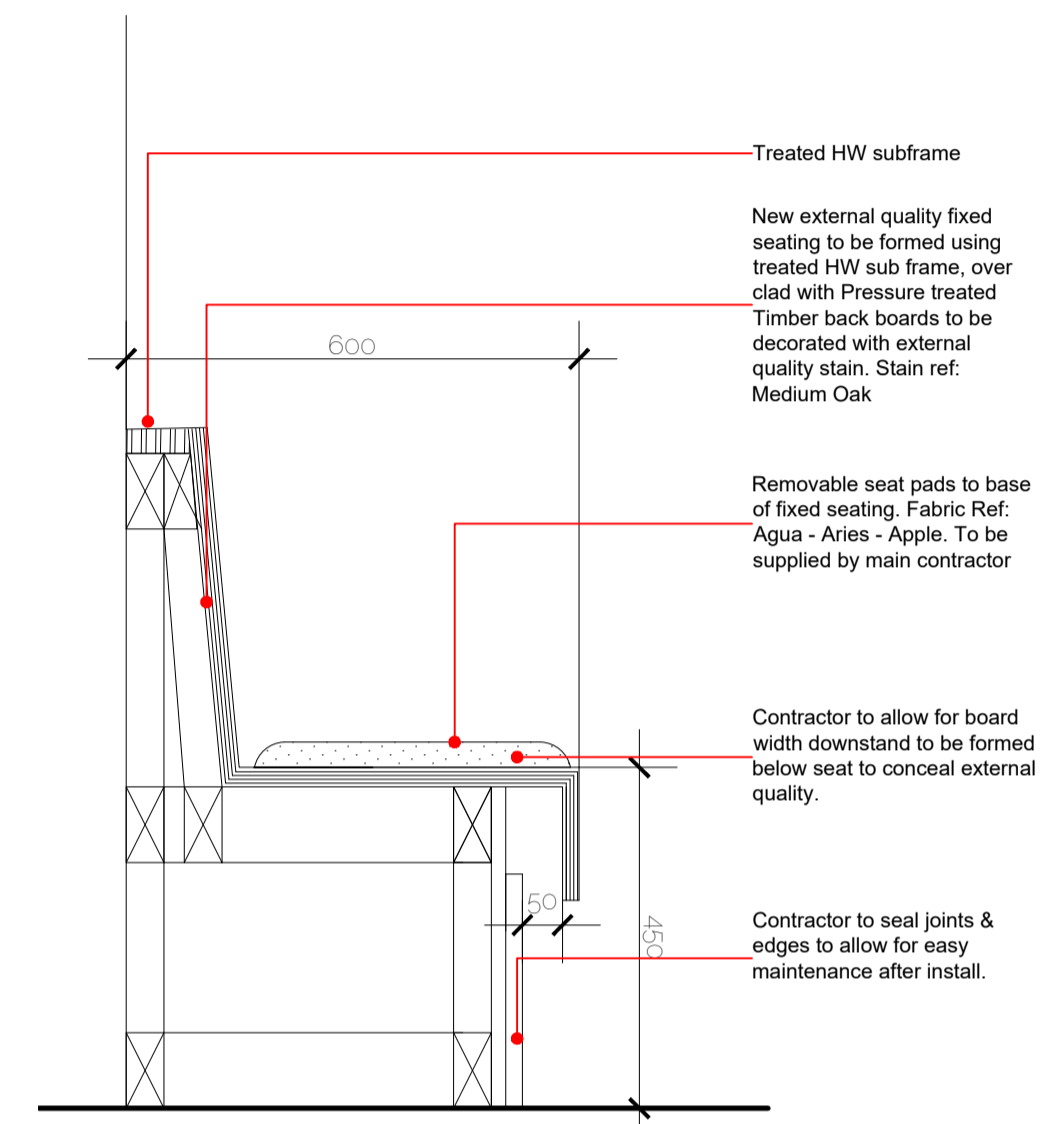
Section B-B Scale 1:10 @ A1
