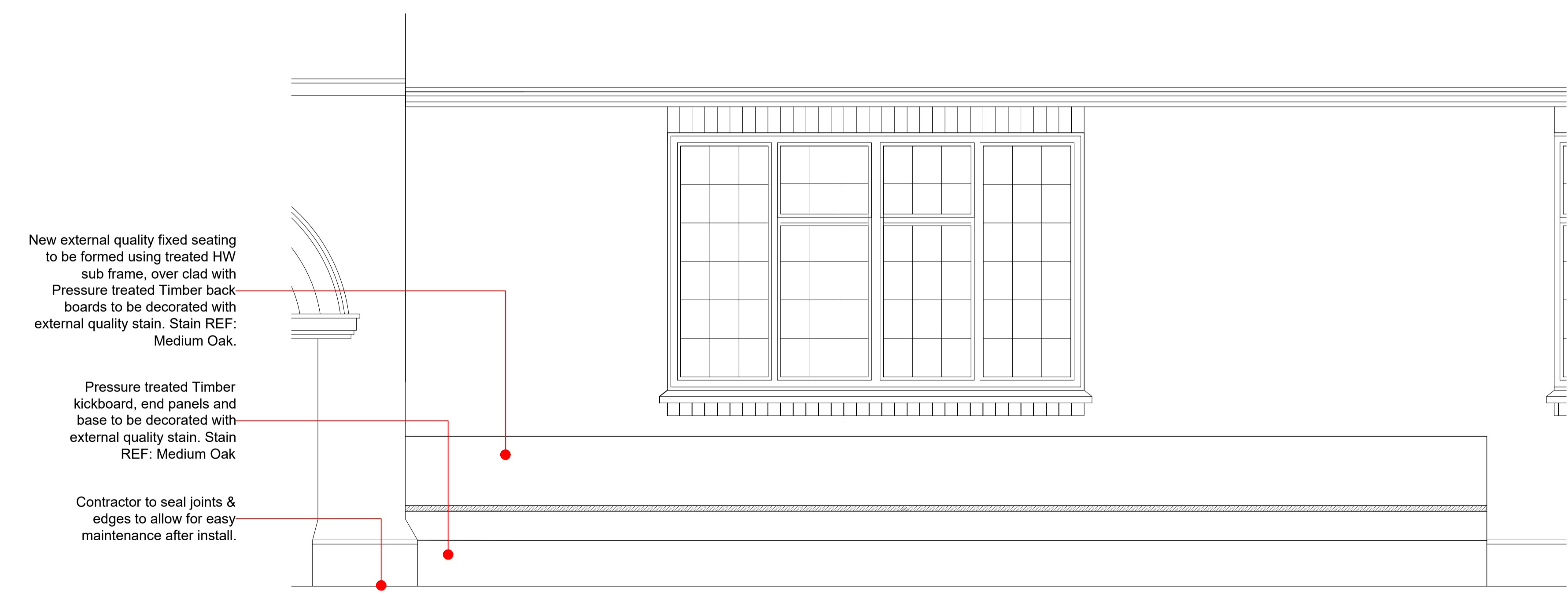
Elevation A-A Scale 1:20 @ A1
