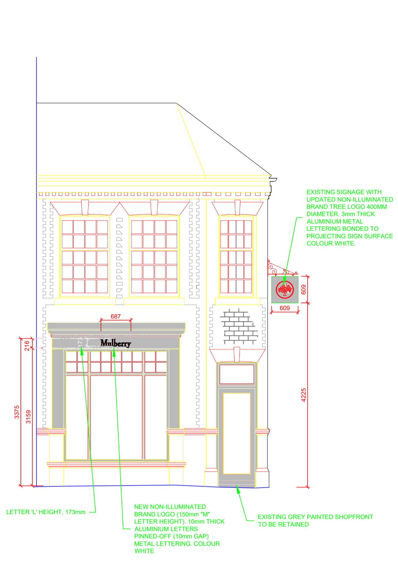
A PROPOSED ELEVATION A. BACK SWINEGATE 1:50 @ A1 1:100 @ A3
